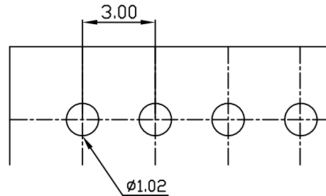
P. C. B Hole Layout
